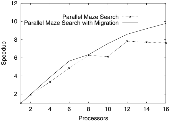
Fig. 7. Speedups for Maze
